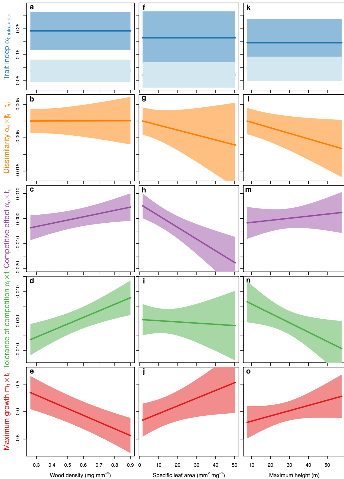
Extended Data Figure 3 | Variation of trait-independent inter and intraspecific competition, trait dissimilarity ( |t_f - t_c| \times \alpha_d ), competitive effect ( t_c \times \alpha_e ), tolerance to competition ( t_f \times \alpha_t ) and maximum growth ( t_f \times m_1 ) with wood density, SLA and maximum height. a–o, Wood density (a–e), SLA (f–j) and maximum height (k–o).
