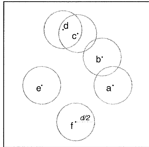
Figure 1: Schematic spatial arrangement of six data points in the plane. Points within a radius d are assigned to the same cluster; hence, points a, b, c, and d are in the same cluster. Points e and f are in separate clusters.
