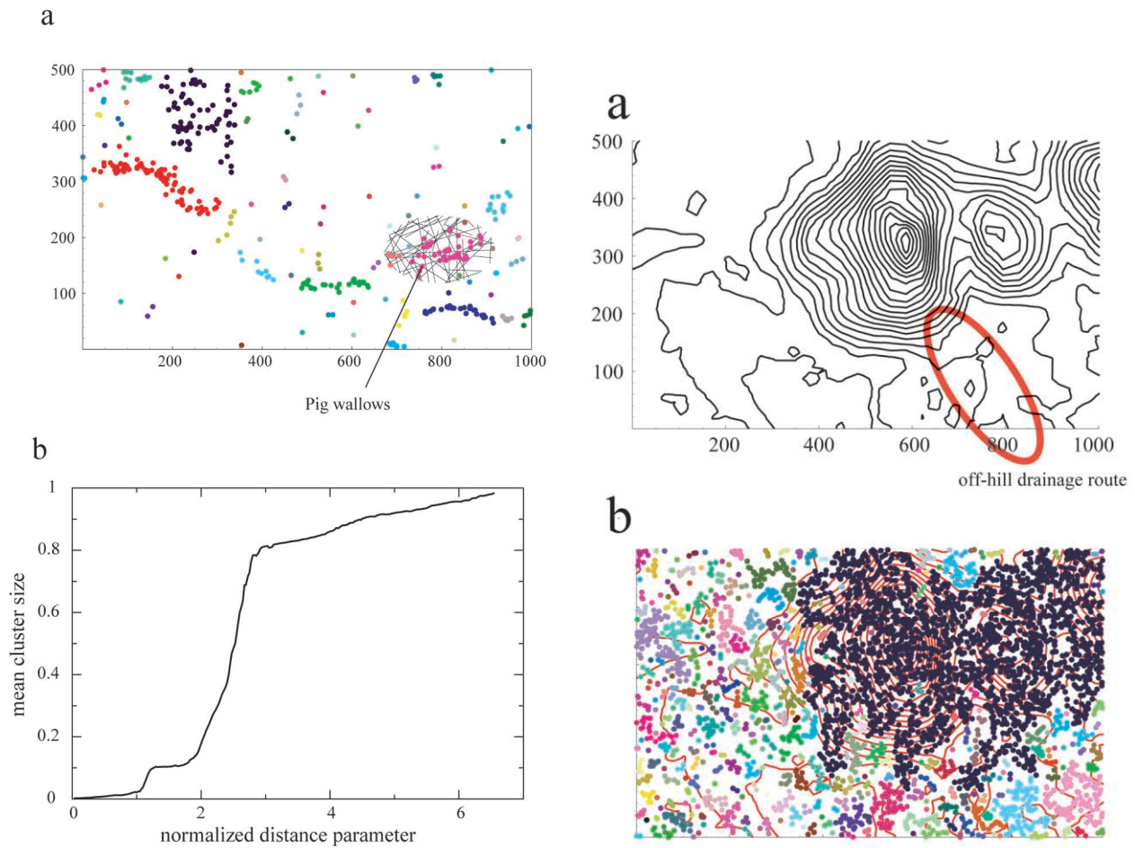
Figure 5: a , Cluster analysis of Pternandra coerulescens that results from the distance parameter d = 25.4 m ( \hat{d} = 1.5 ). There are 438 stems within the plot, which form 79 clusters. Most of the clusters of P. coerulescens are linear in shape. The arrow indicates the locations of pig wallows within the 50-ha plot. b , Mean cluster size curve for P. coerulescens . The algorithm was run with a positive temperature ( \chi = 0.08 ) to minimize finite size effects. The resulting curve shows two principal transitions.
