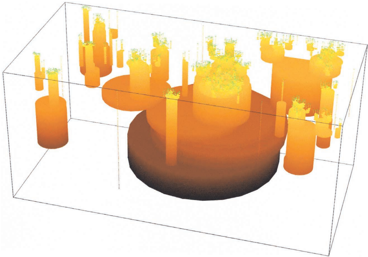
Figure 4: Dependence of clusters on the distance parameter d for Mallotus penangensis . The figure shows a three-dimensional graph of M. penangensis clusters. The X- and Y-axes of the figure correspond to the length and width of the 50-ha plot, as in figure 3a. The Z-axis corresponds to the value of d . The color also corresponds to the value of d . On the upper plane, d = 0 , and each tree forms its own cluster, all plotted in green. As d increases down the Z-axis, larger clusters form. Each cluster is represented in the figure by a circle centered at the center of mass of the cluster. The radius of the circle equals the mean distance of the trees in the cluster to its center of mass.
