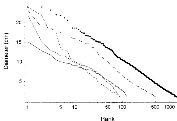
Figure 9: Distribution of tree diameters within the four largest Mallotus penangensis clusters, compared with the distribution of M. penangensis diameters in the entire 50-ha census (large dots). The figure shows a rank dbh plot on a semilogarithmic axis. The individual clusters of M. penangensis exhibit nearly the same full range of dbh classes as the 50-ha plot as a whole.
