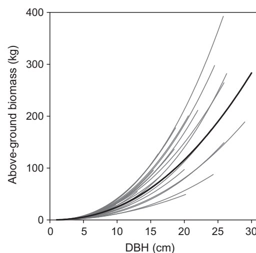
Fig. 1. Allometric relationships between DBH and above-ground biomass (AGB) of the 26 studied species. Thin lines are species-specific allometric regression models (Table 1). Bold line corresponds to mixed-species allometric regression model 1 (Table 3). Back-transformed data are presented.
