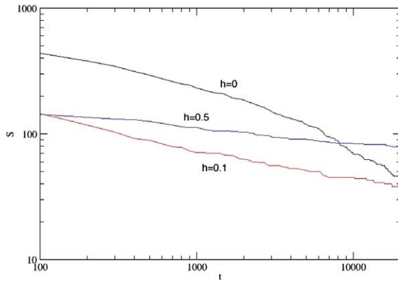
Fig. 4. Without speciation. Dynamics of the number of species S when the speciation rate is \nu=0 , starting from high-diversity configuration ( \nu=10^{-4} ). Habitat preference slows the rate of species loss. The examples are from continuous habitat preference, with \sigma=2 . Other cases were similar.
