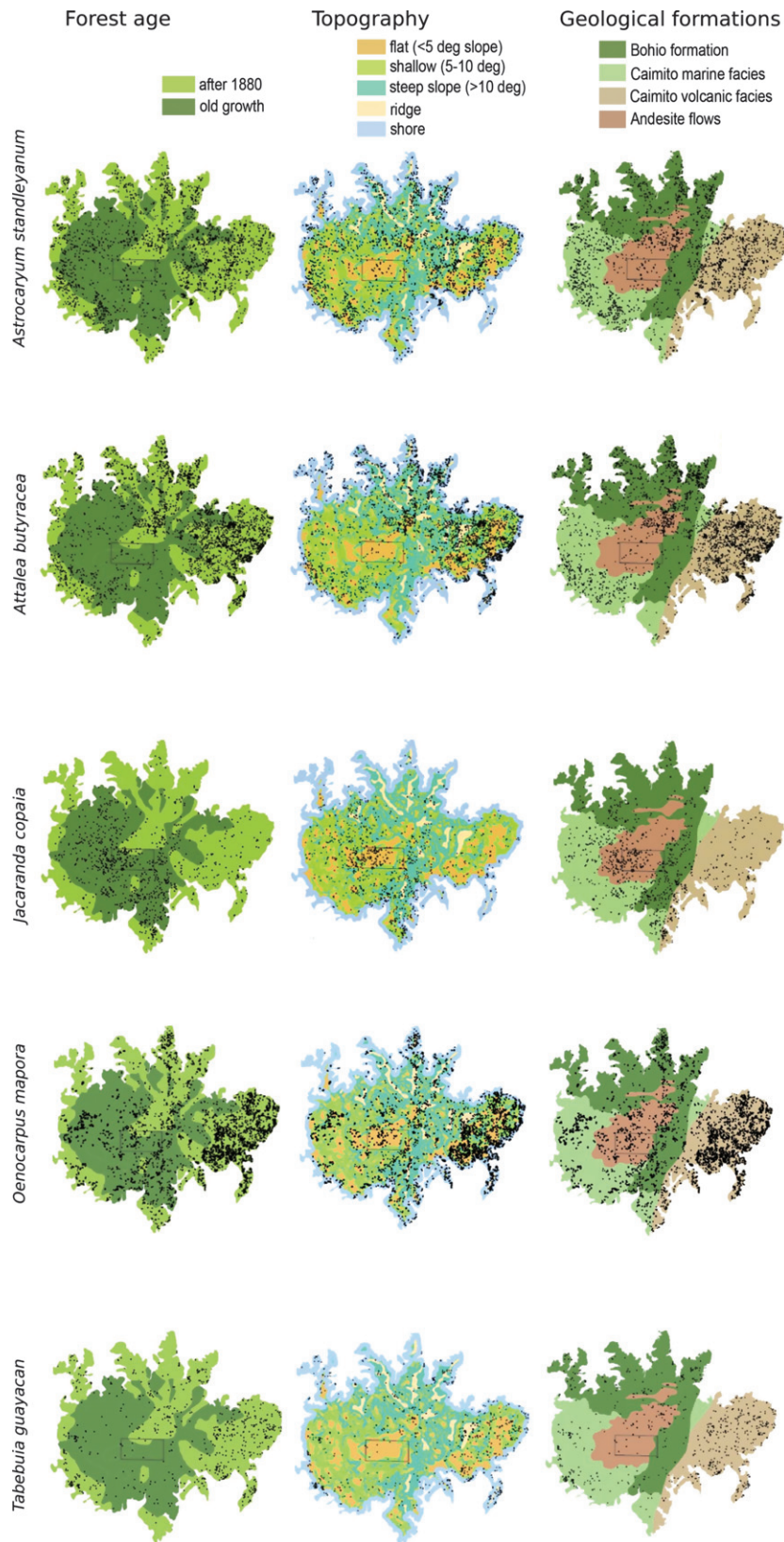
Fig. 1. Spatial distribution of five tropical tree species on Barro Colorado Island, Panama, in relation to environmental factors.
