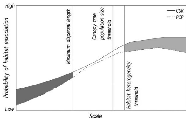
Fig. 4. Strength of habitat associations based on comparison to a complete spatial randomness (CSR) model. Habitat associations were determined using an observed vs expected approach based on comparison to 1000 CSR simulations for each level of the evaluated environmental variable. Strength of the relationship was measured as the number of the 1000 contrasts where observed occurrence on a certain habitat was higher than the expected occurrence on that habitat. Box plots summarize the median and interquartile variability across replicates at a particular sampling scale. Numbers of replicates per scale are 10 for 50 and 100 ha, six for 200 ha, three for 400 ha, and one for 800 and 1600 ha.
